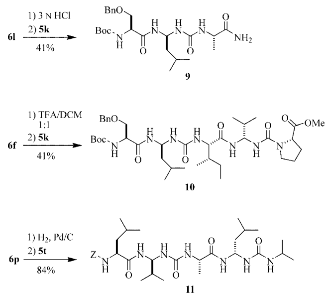
Scheme 3. Solution-phase synthesis of oligo(amide/urea) hybrids.
