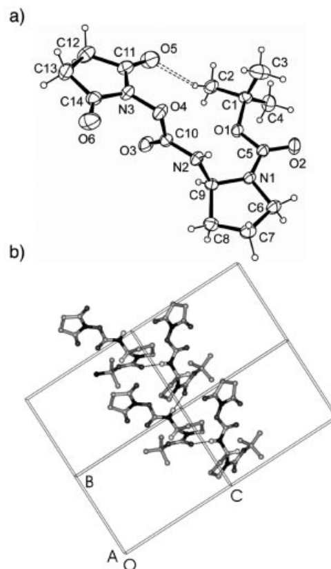
Figure 2. Ortep diagram (a) and partial crystal packing (b) of 4f .
