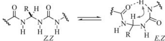
Figure 6. Representation of the extended ( trans,trans ) and folded ( cis,trans ) conformations adopted by the urea linkage in ureido-peptides. The strong NOE connectivity between the \alpha -CH( i ) and NH( i +1), characteristic of the ( cis,trans ) conformation observed in solution, is shown by an arrow.
