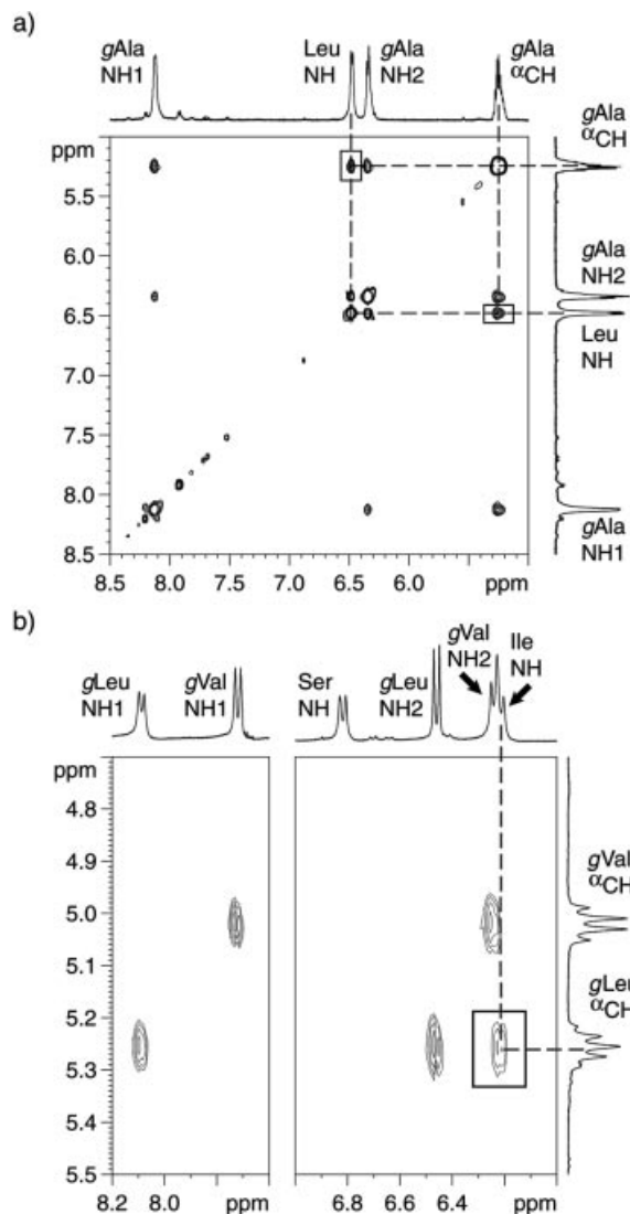
Figure 5. Parts of the ROESY spectra demonstrating the cis,trans conformation of the N,N' -disubstituted urea fragment in a) 6i and b) 10 , at 298 K in [D_5] pyridine and [D_6] DMSO, respectively.
