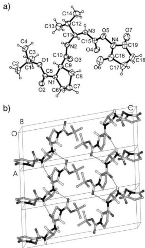
Figure 3. Ortep diagram (a) and partial crystal packing (b) of 5f .
