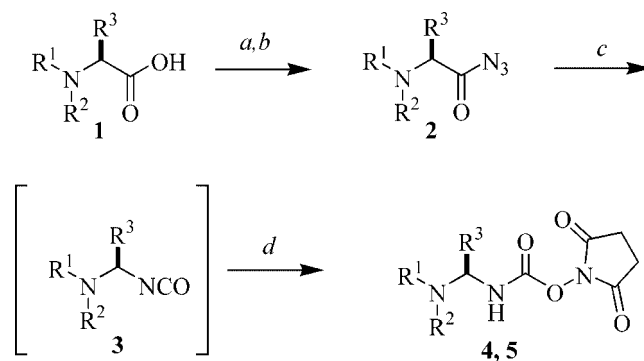
Scheme 1. a : EtOCOC 2 H 5 , NMM, THF, -20 °C; b : NaN 3 , H 2 O; c : toluene, 65 °C; d : N -hydroxysuccinimide, pyridine.
