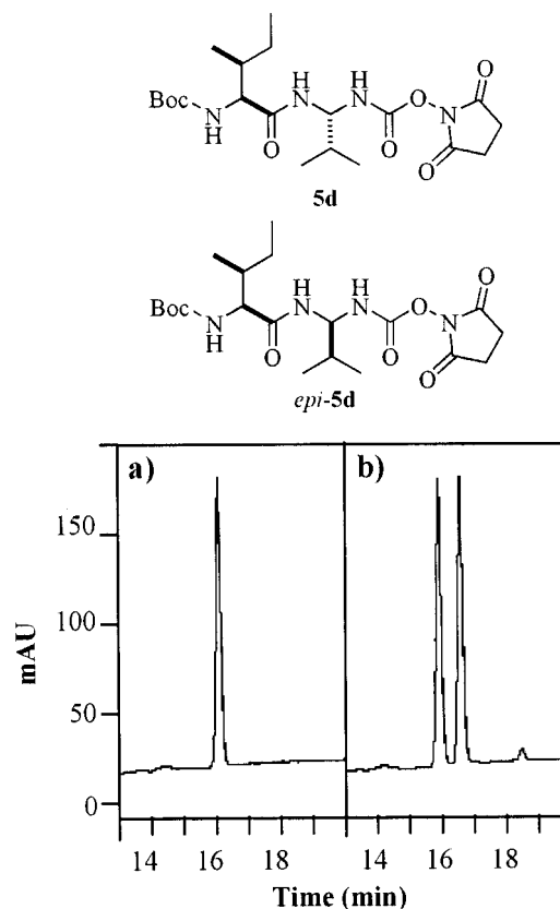
Figure 1. C 18 RP-HPLC traces of crude 5d (left panel) and an equimolar mixture of 5d and epi - 5d (right panel).
