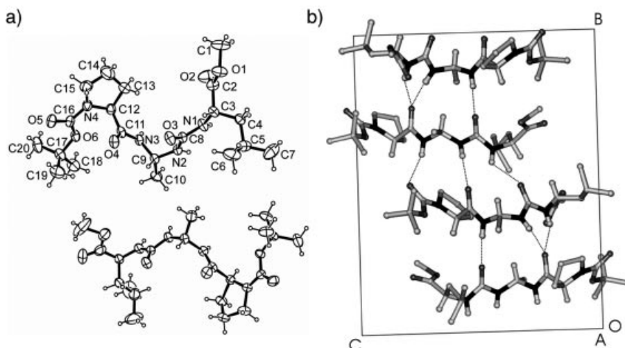
Figure 4. Ortep diagram (a) and partial crystal packing (b) of 6i .
